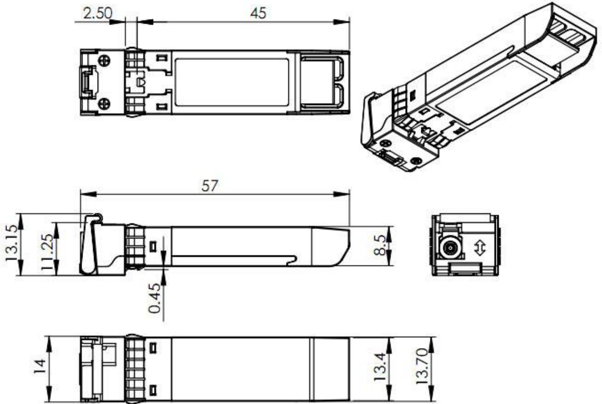
Mechanical Drawing
